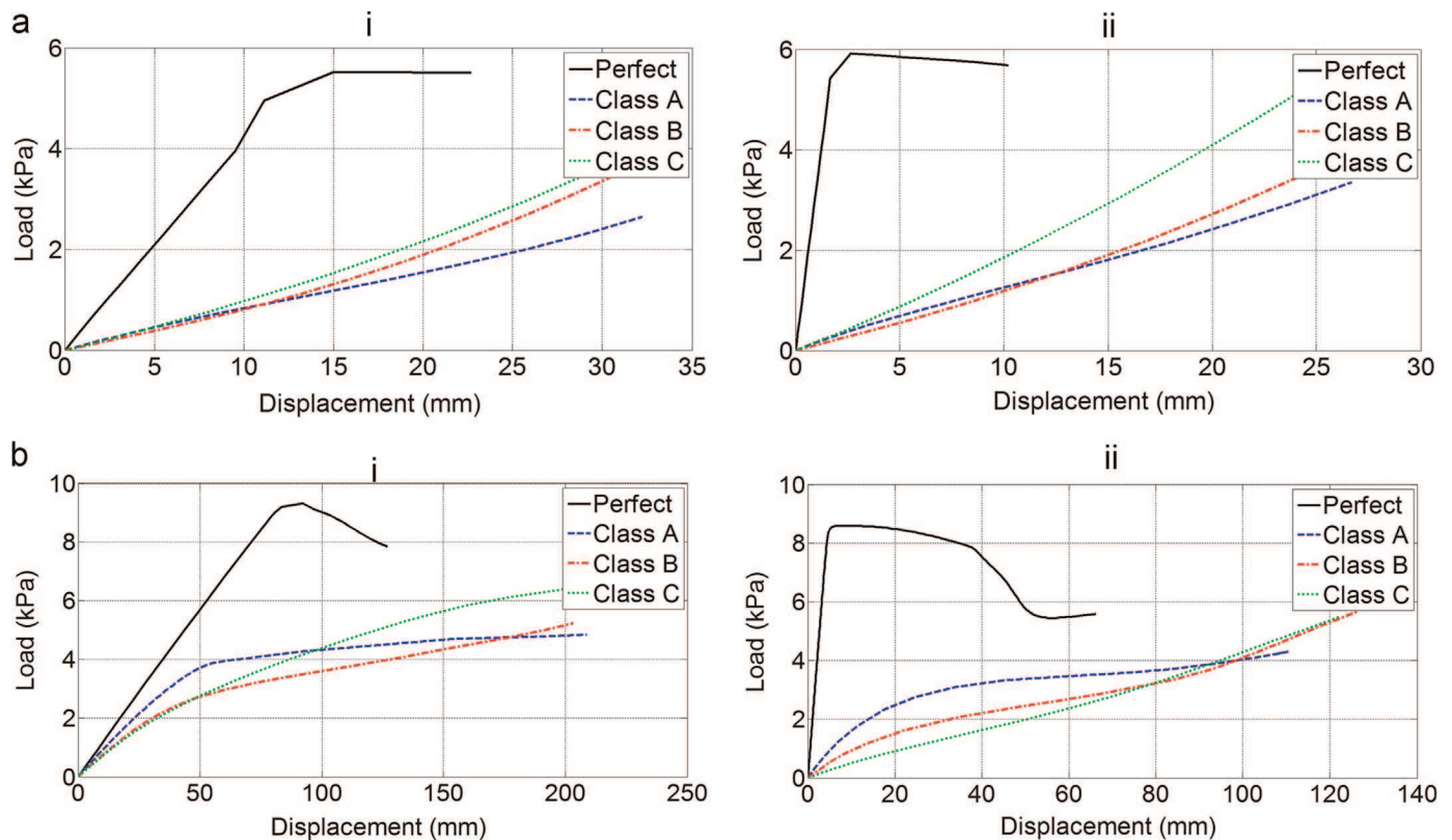
Fig. 7. GNIA load-displacement curves; (a) T-776 for EN1993-1-6 wind pressure (i) and uniform wind pressure (ii); (b) T-761 for EN1993-1-6 wind pressure (i) and uniform wind pressure (ii).
