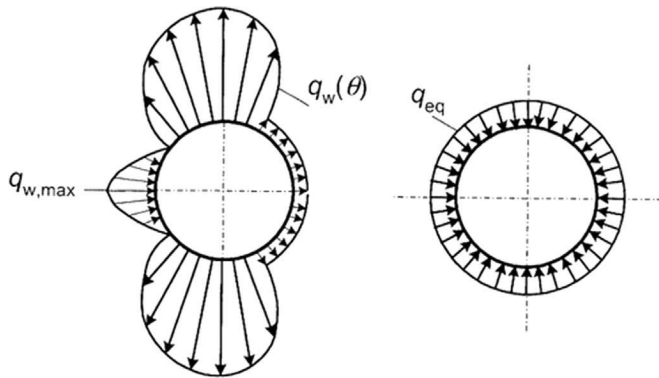
Fig. 3. Distribution of wind pressure on cylindrical tanks (left) and equivalent uniform pressure (right).
