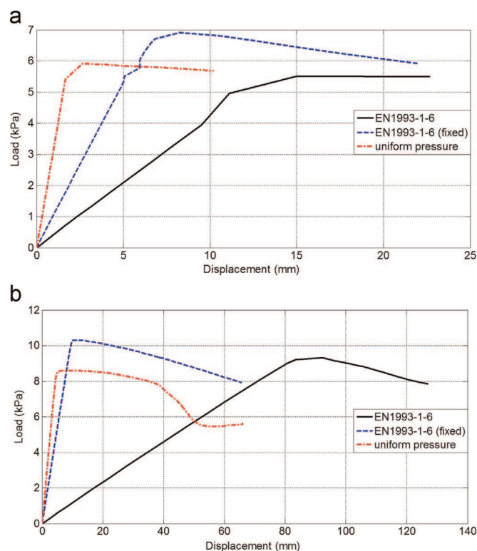
Fig. 6. GNA load-displacement curves; (a) T-776; (b) T-761.
