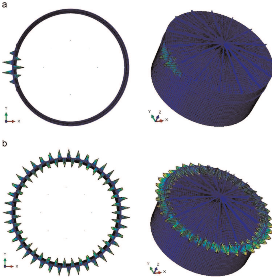
Fig. 4. Buckling deformation modes for tank T-776; (a) Wind pressure distribution according to EN1993-1-6; (b) Uniform wind pressure distribution.
