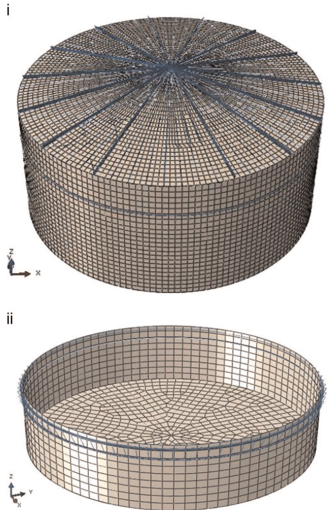
Fig. 2. Simulation of T-776 (i) and T-761 (ii) with the FEM.
