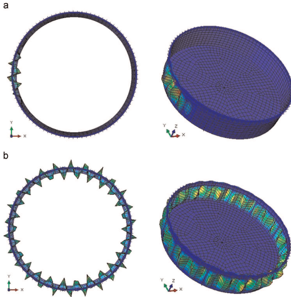
Fig. 5. Buckling deformation modes for tank T-761; (a) Wind pressure distribution according to EN1993-1-6; (b) Uniform wind pressure distribution.
